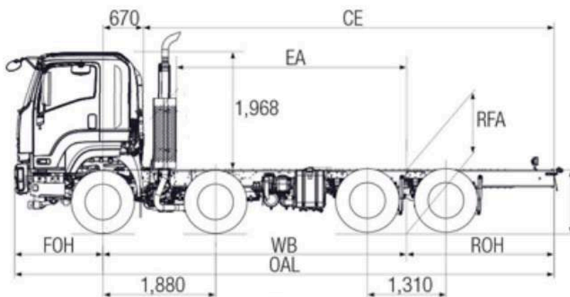
FYH350S shown
