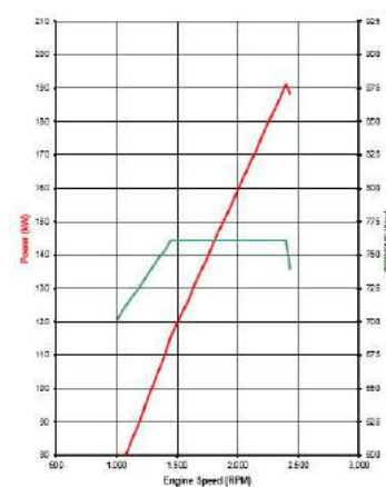
Isuzu 6HK1-TCC
