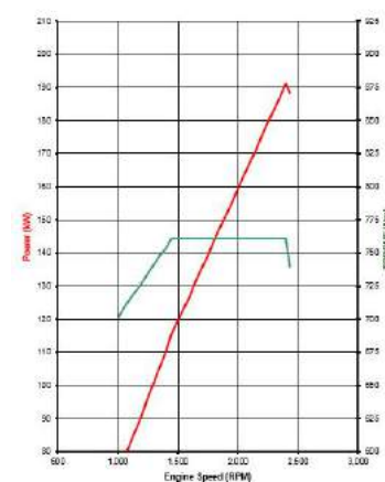
Isuzu 6HK1-TCC
