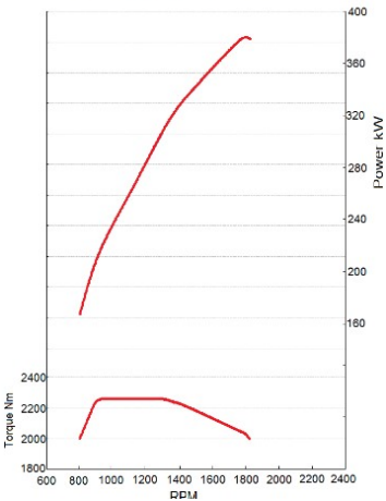
Engine Performance Curve 6WG1 TCS
