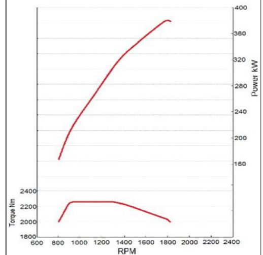
Engine Performance Curve 6WG1 TCS
